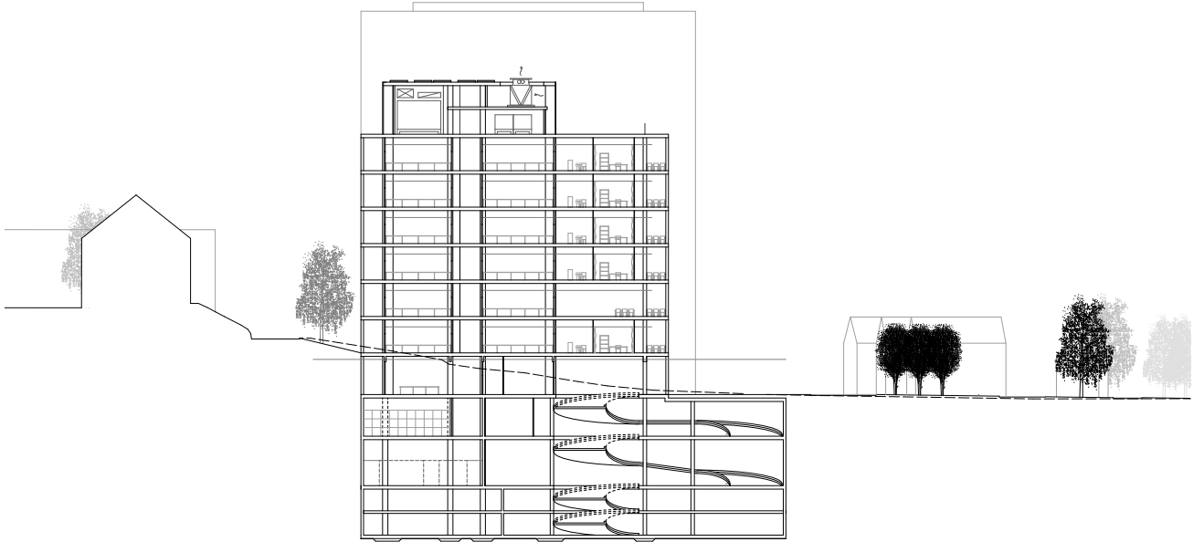
Cross Section
