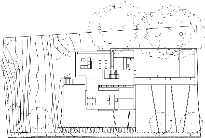
Ground floor plan | The fluid spaces allow spacious living experience
