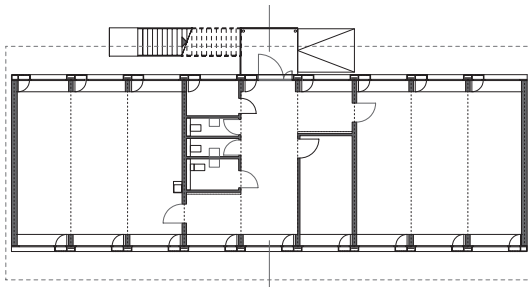
PLAN GROUND FLOOR
