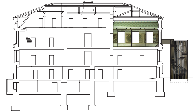
SECTION | A NEW ELLIPTICAL STAIRCASE MEETS THE REQUIREMENTS FOR EMERGENCY EVACUATION
