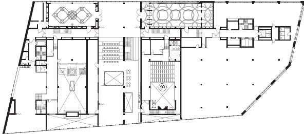
Plan +2 House of Religions
