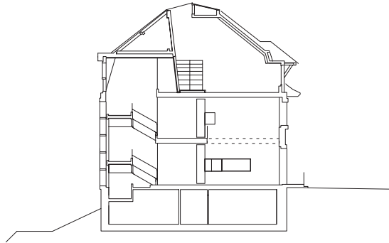
SECTION I | A SPACE OVER 2 FLOORS OFFERS VOLUME TO THE ENTRANCE AREA
