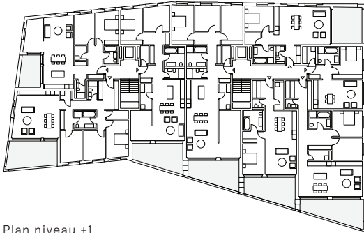
Plan niveau +1
